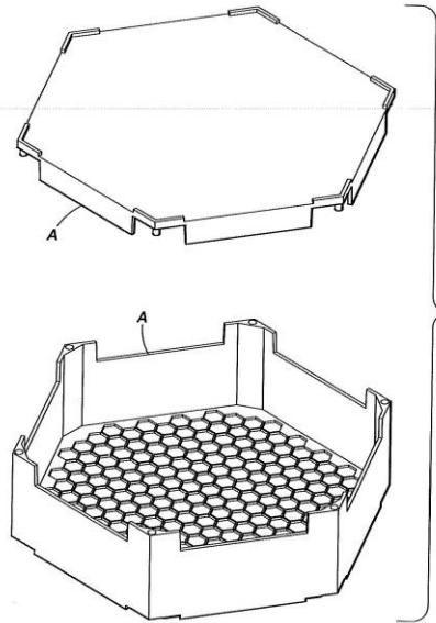
TOP PERSPECTIVE VIEW OF ARTICLE IN AN EXPLODED CONFIGURATION
